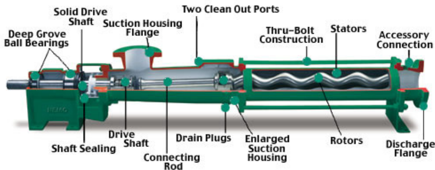
FIGURA 8.3: Bomba helicoidal.
